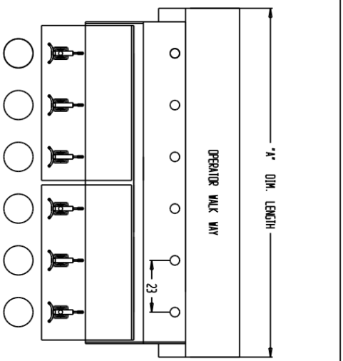
TP VIEW
